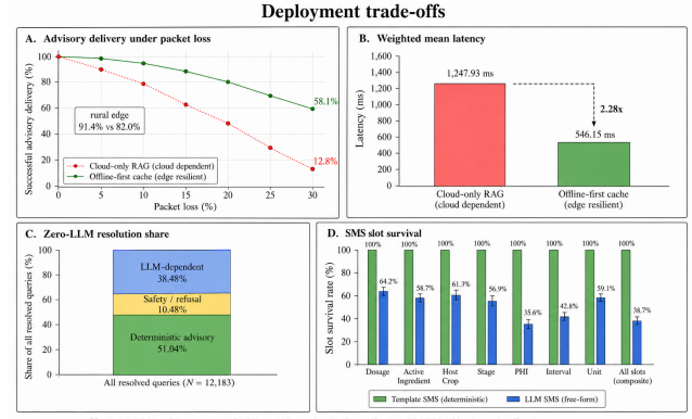
Figure 6: Deployment Trade-offs: Systems Efficiency, Connectivity Resilience, and Channel Economics. (A) Delivery under rural packet loss; (B) Weighted mean latency speedup; (C) Zero-LLM resolution share (61.5%); (D) 160-character Bengali SMS slot survival rate.
