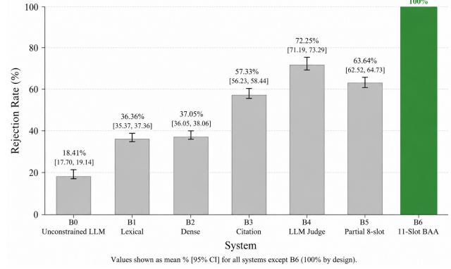
Figure 3: Metamorphic Rejection Rates under 11,000 Systematic Corruptions per System (Layer E28). BAA achieves 100.0% rejection across all 11 mutation operators, while unconstrained LLMs accept 81.59% of corrupted advice.
